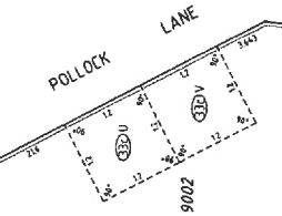
ENLARGEMENT 'V' NOT TO SCALE
